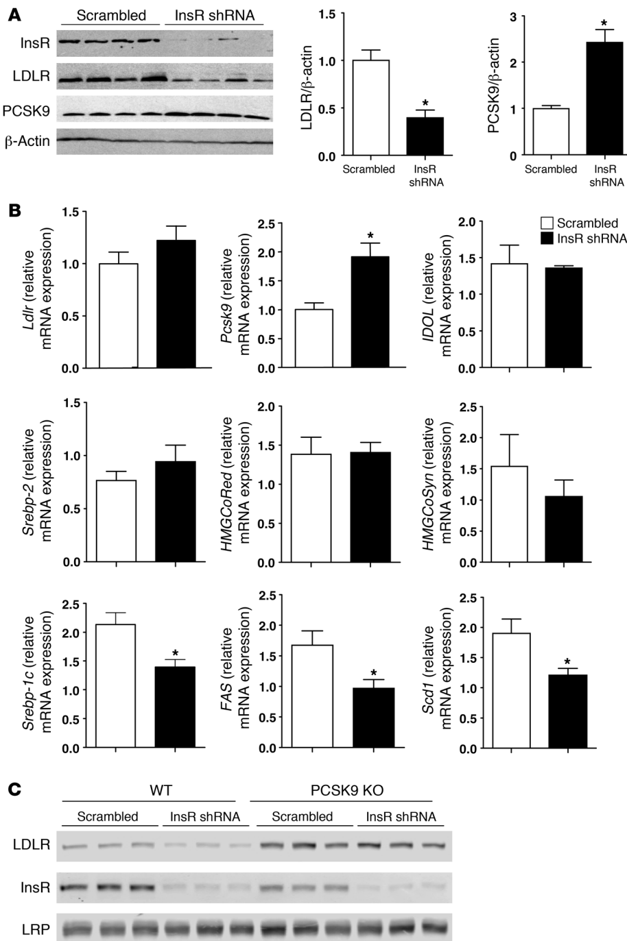
Figure 1 Effect of hepatic InsR knockdown in C57BL/6 mice. (A) Mice 10–11 weeks of age were injected with the InsR shRNA adenovirus and sacrificed on the 11th day after injection. Immunoblot analysis of InsR, LDLR, PCSK9, and \beta -actin in liver lysates from mice after infection with scrambled control adenovirus or InsR shRNA. Livers were collected after a 5-hour fast. Each lane shows the liver lysate of a different mouse. Right panel: Quantification of the Western blot results. (B) Analysis of hepatic gene expression by real-time qPCR in scrambled or InsR shRNA adenovirus-infected mice. (C) Membrane fraction of liver extract was prepared from Pcsk9 knockout or WT mice after infection with scrambled control adenovirus or InsR shRNA and subjected to Western blot analysis of LDLR, InsR, and LRP. n = 4 –5 mice per group. * P < 0.05 .
